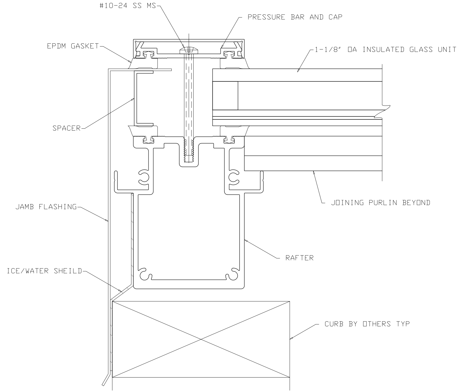
4 JAMB SECTION SCALE 1' - 0" = 1' - 0"
